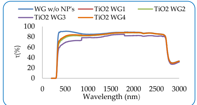
Figure 10a. SW transmittance using TiO 2 - SiO 2 on conventional WGs
